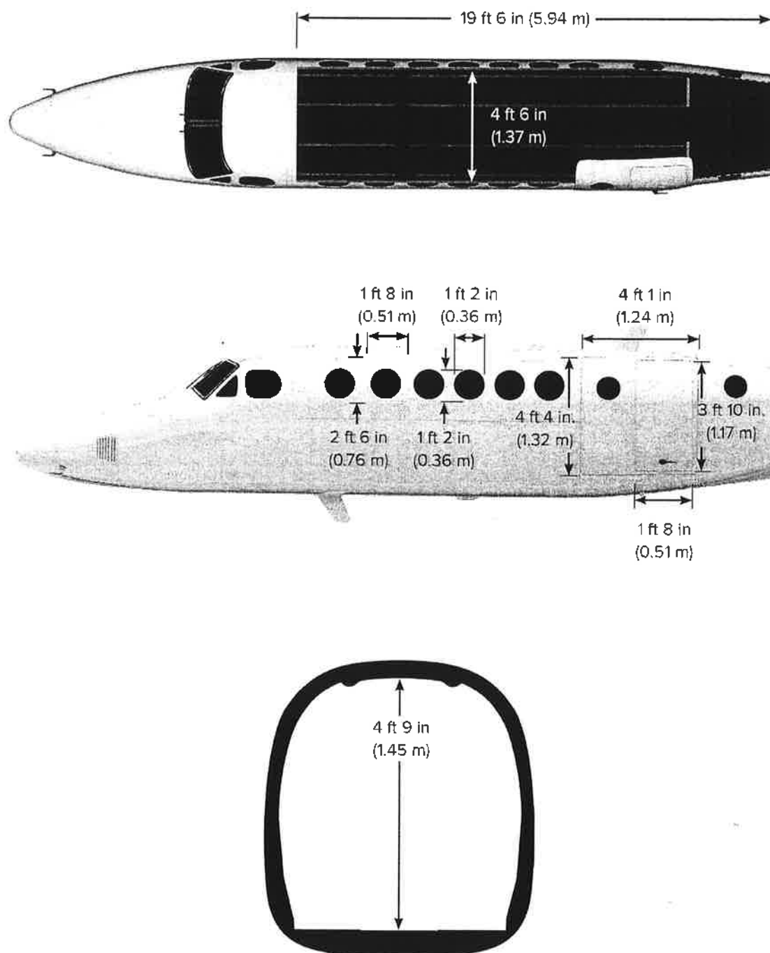
Figure 2: Interior Dimensions
