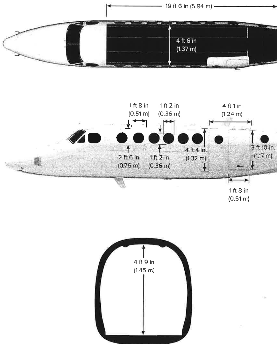
Figure 2: Interior Dimensions
