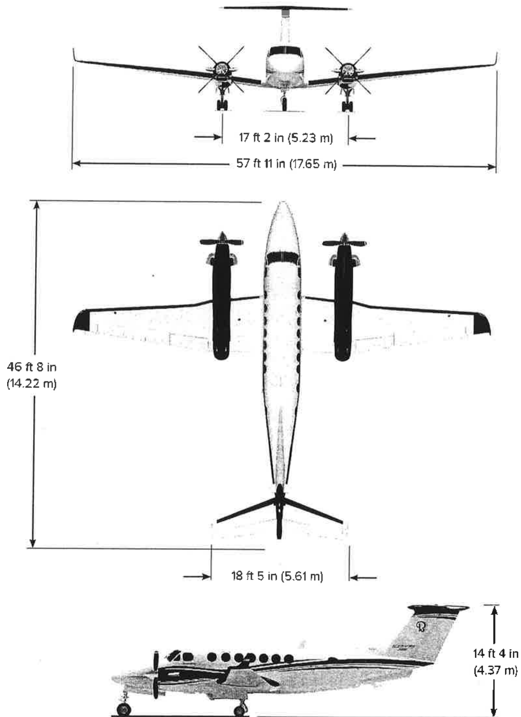
Figure 1: Exterior Dimensions
